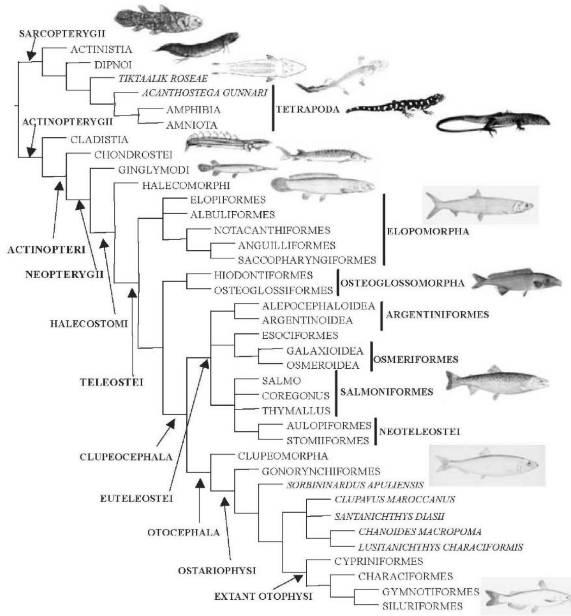
Figure 4 Relationships among the major osteichthyan groups examined, derived from the “majority fools” tree obtained in the cladistic analysis of Chapter 3 (see Fig. 3).
