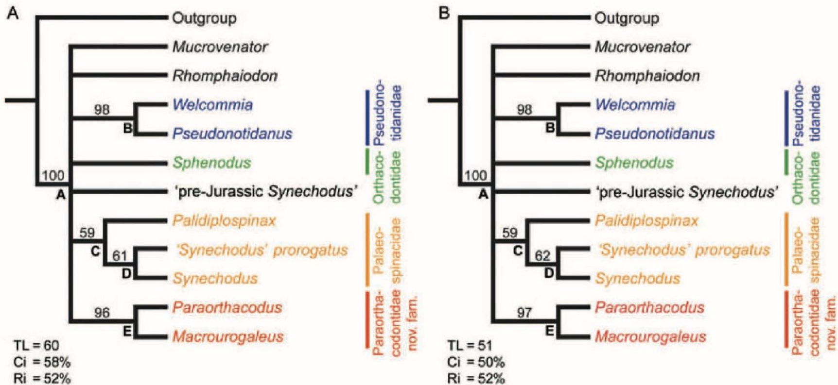
Fig. 4 A, B. Phylogenetic hypothesis of synechodontiform sharks excluding (A) and including (B) uninformative characters, conducted by using heuristic search with tree-bisection-reconnection of branch-swapping. Strict consensus trees of both 16 equally most parsimonious trees; numbers above branches are bootstrap estimates. For character distribution and corresponding character states based on DELTRAN or ACCTRAN optimization, see Appendix S8.
