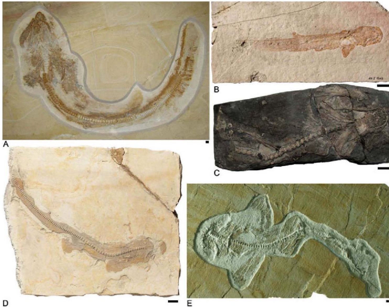
Fig. 1 A–E. Holomorphic specimens of synechodontiform taxa. —A. † Paraorthacodus jurensis (SMNS 88987/1). —B. † Macrourogaleus bassei (BSPG AS 1363, holotype). —C. † Palidiplospinax enniskilleni (NHML P.3189, holotype). —D. † Synechodus sp. (BSPG 1878 VI 6). —E. † Sphenodus mucer (SMNS 80142/44). Scale bars equal 1 cm.
